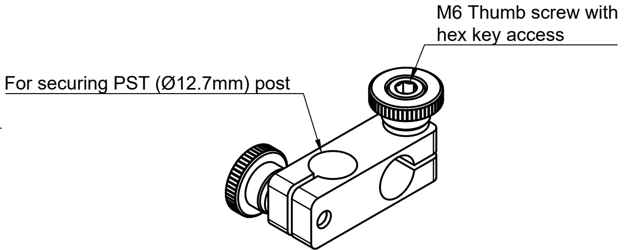
Right angle post clamp to join PST (Ø12.7mm) post at 90°
