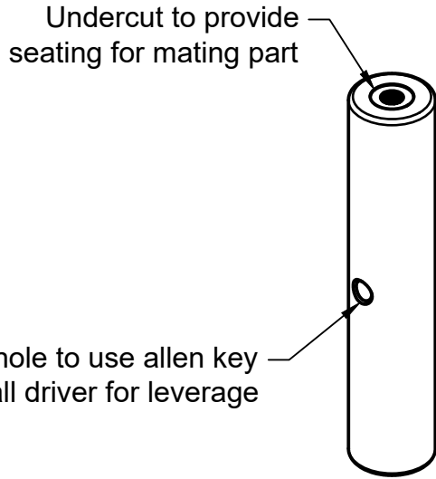
Stainless steel extension post
